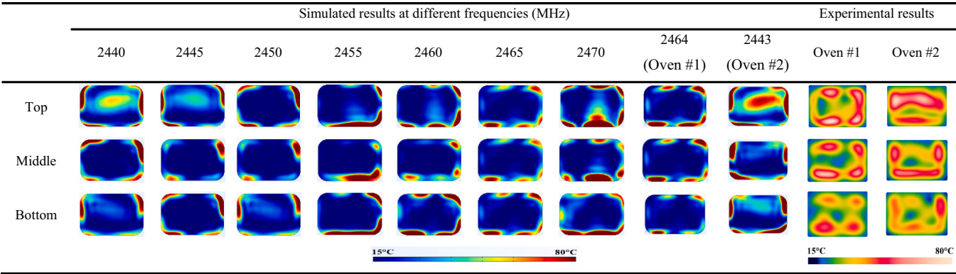
Fig. 7. Experimental and simulated heating patterns of whey protein gel (135 mm \times 92 mm \times 22 mm) heated in two magnetron-based microwave ovens (#1, #2). The experimental heating patterns of three layers were obtained by a thermal camera. Oven #1 had a measured peak frequency of 2464 MHz, while oven #2 had a measured peak frequency of 2443 MHz (Fig. 6).
