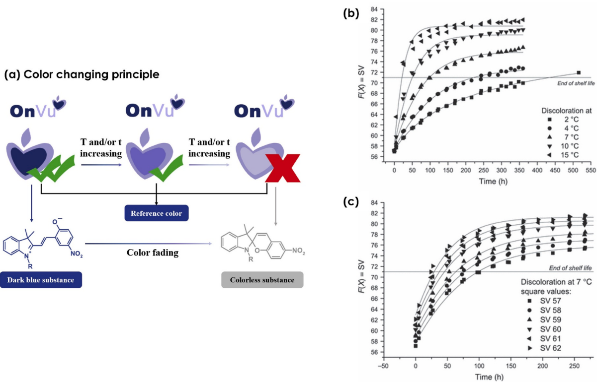
Fig. 4. (a) Principle of photochromic OnVu TTI, color changing kinetics at (b) different temperatures, and (c) different UV charging times (Kreyenschmidt et al., 2010).
