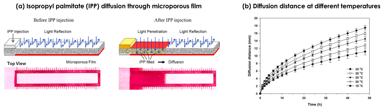
Fig. 3. (a) Principle of diffusion-based TTI and (b) temperature-dependent diffusion kinetics (Kim et al., 2016).
